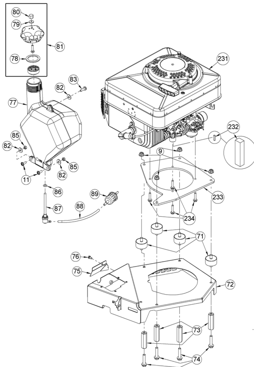
Motor und Tank AS 531/2T MK-Kat
