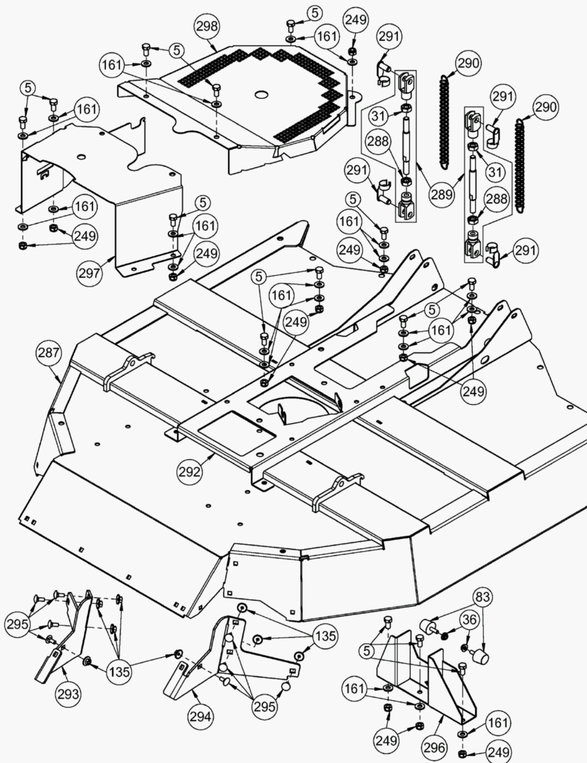
Messerhaube AS 940
