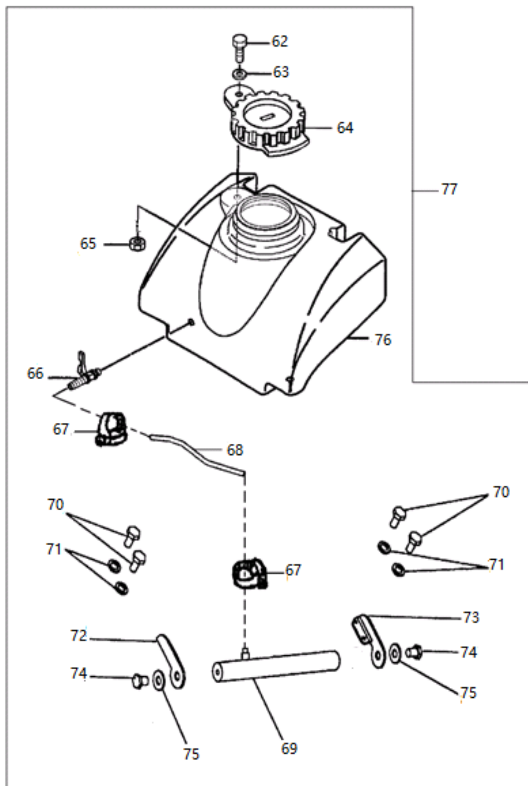
MS60 PARTS LIST 3
