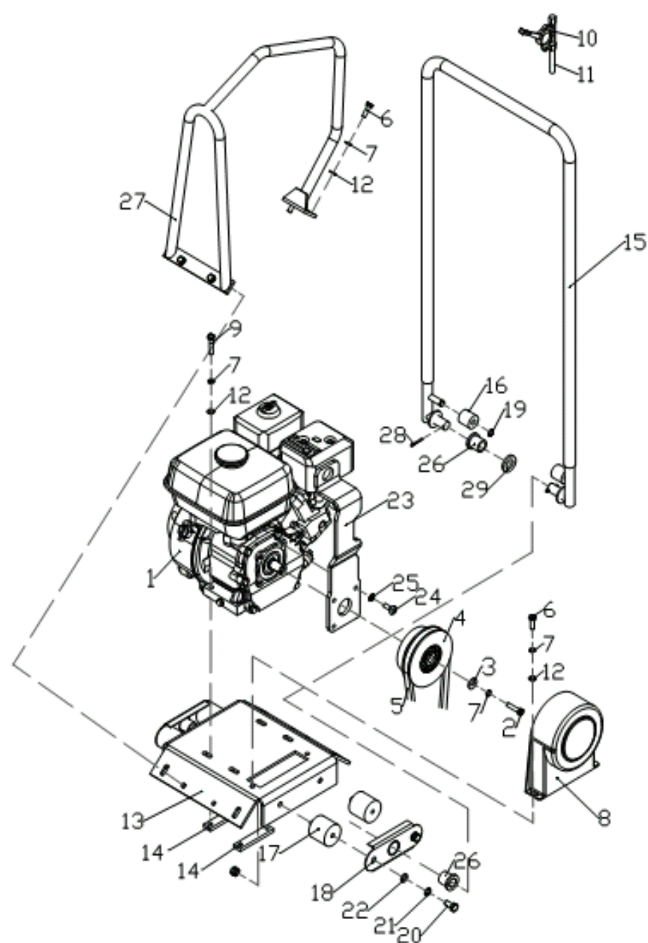
MS100 PARTS LIST 1
